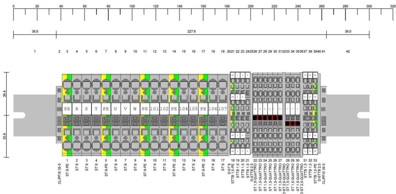
Figure 19. Distribution board
